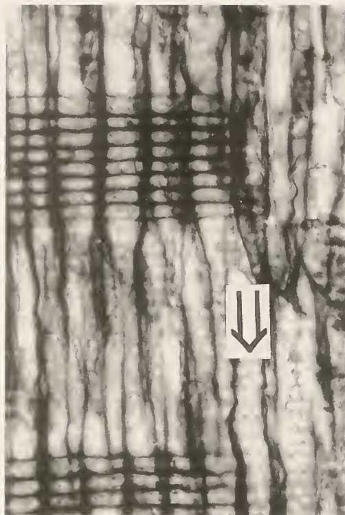
Fig. 4. Taxodioxyton sp., Mine Bílina, No. 2. Longitudinal radial section; radial tracheid walls with opposite (arrow) pits and cross field pitting. \times 90 .
